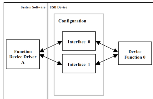
Figure 44. Multiple Interfaces with Single Function
