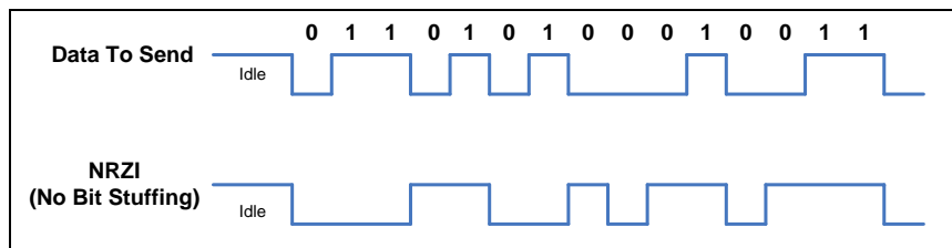
Figure 9. Data to NRZI Encoding
