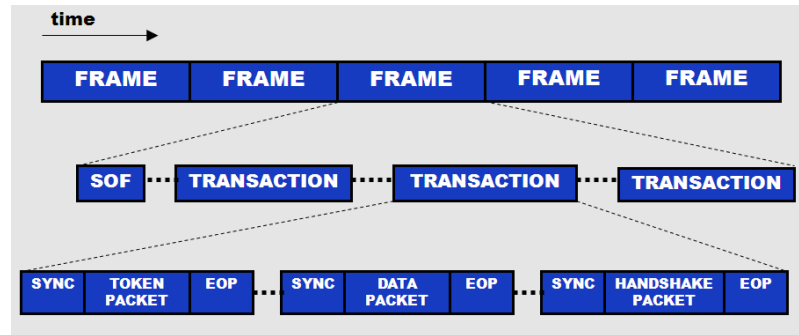
Figure 22. USB Communication from a Time Perspective
