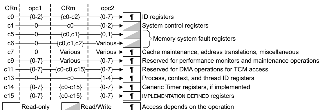
Figure B5-3 CP15 register grouping by primary coprocessor register, CRn, PMSA implementation
