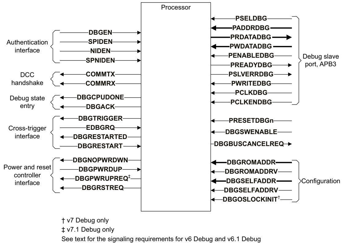
Figure A-1 Recommended external debug interface, including APB3 slave port
