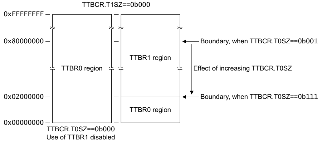
Figure B3-18 Control of TTBR boundary, when TTBCR.T1SZ is zero
