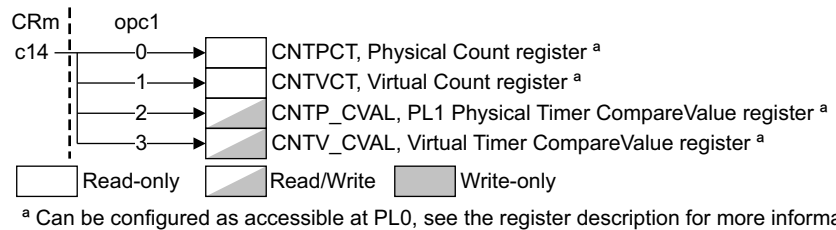
Figure B5-12 CP15 64-bit c14 registers in a PMSA implementation that includes the Generic Timer Extension
