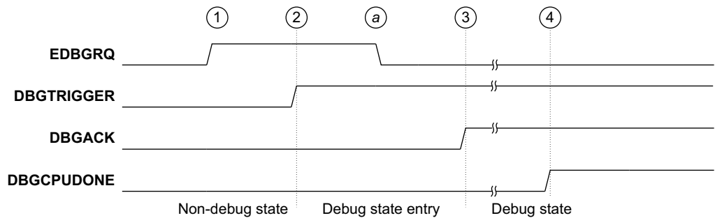
Figure A-2 Signaling for Debug state entry on an External debug request
