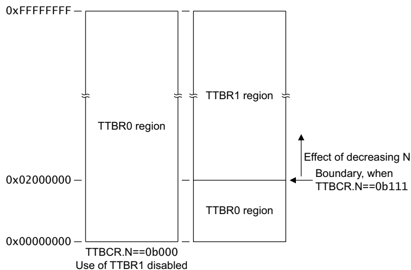
Figure B3-6 How TTBCR.N controls the boundary between the TTBRs, Short-descriptor format
