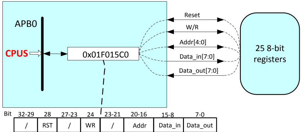
Figure 4-16. Audio Codec Analog Register Diagram
