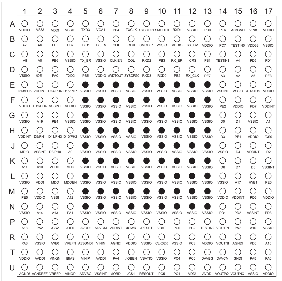
Figure 32-1. Ethernet Option Pinout Looking Through the Top of Package
