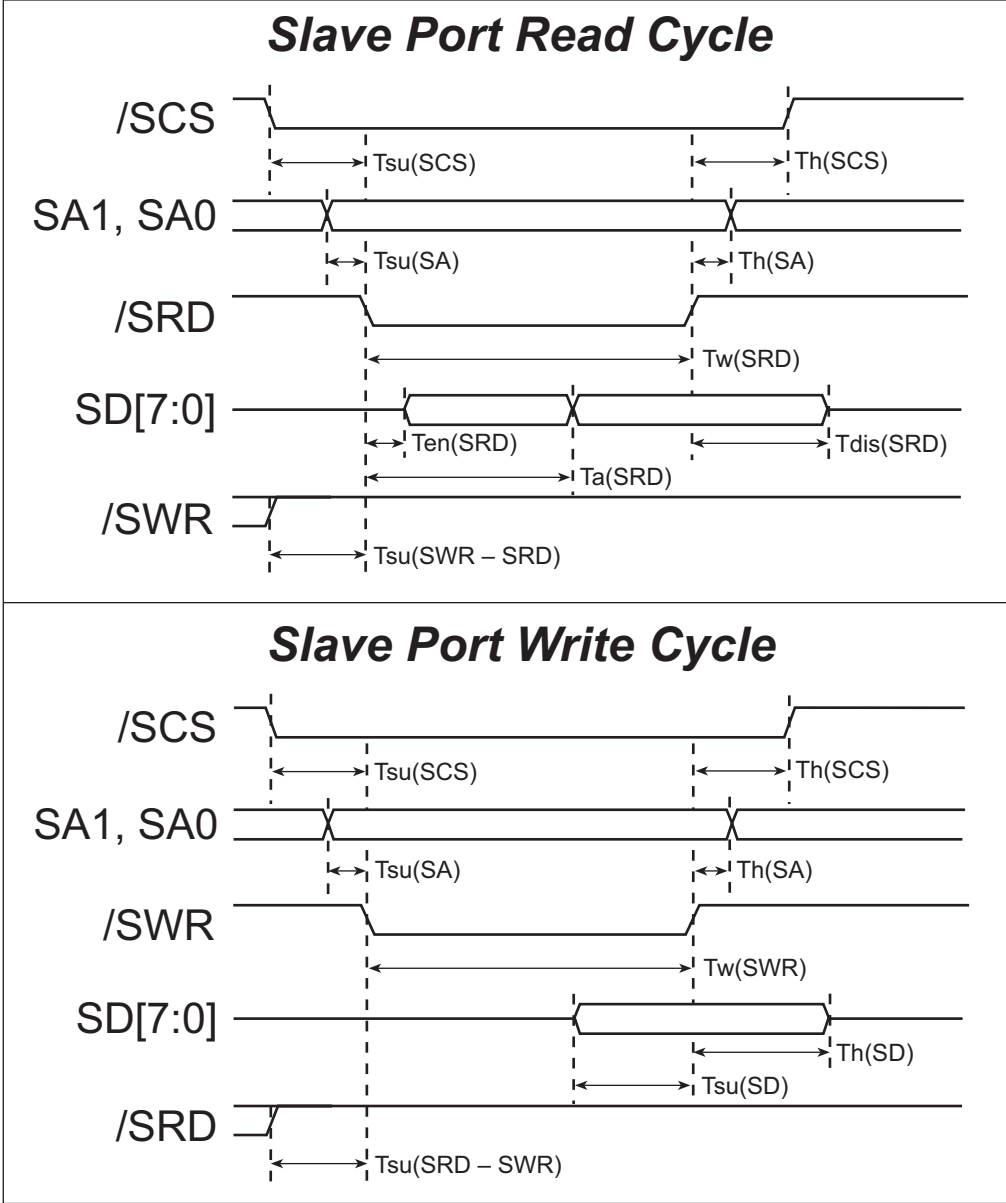
Figure 19-2. Slave Port R/W Timing Diagram
